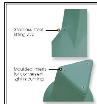
Detail of the PB700 lifting eye, and lantern mounting inserts.
